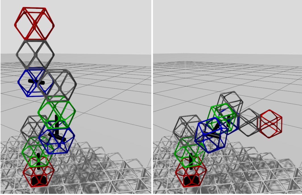
Figure 6.3: Validation of reachable configuration of a robot, initial and target pose
