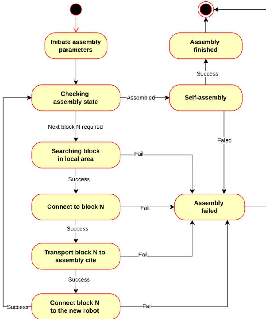
Figure 4.3: State chart of self-replication assembly process
