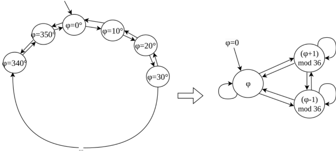
Figure 4.6: Robot block transition system for angle \phi
