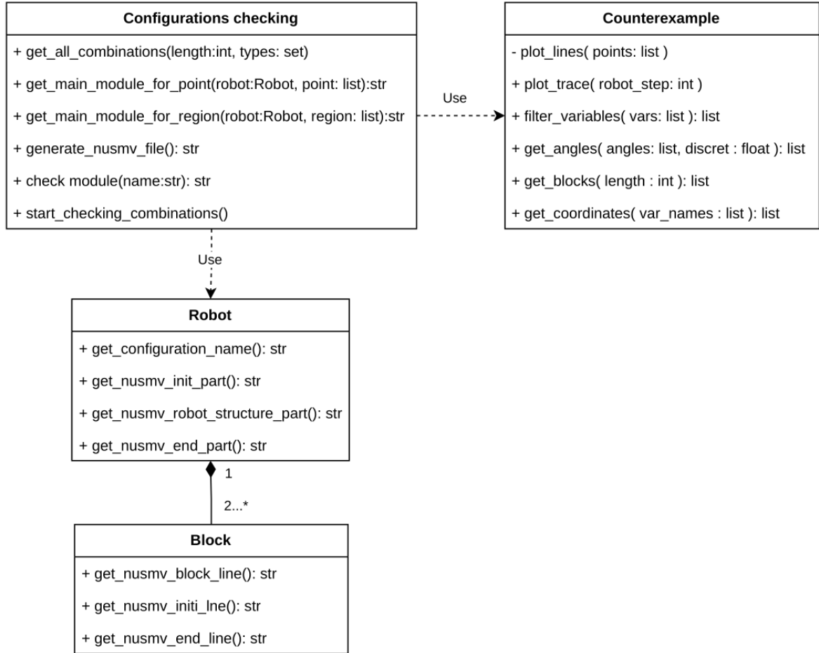
Figure 4.14: Class diagram of configuration checking, searching for feasible configurations
