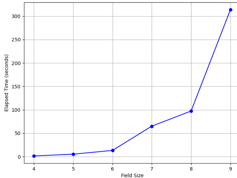
Figure 6.6: Model checking time with field size
