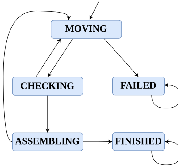
Figure 4.10: Simplified transition system relative to robot_state variable
