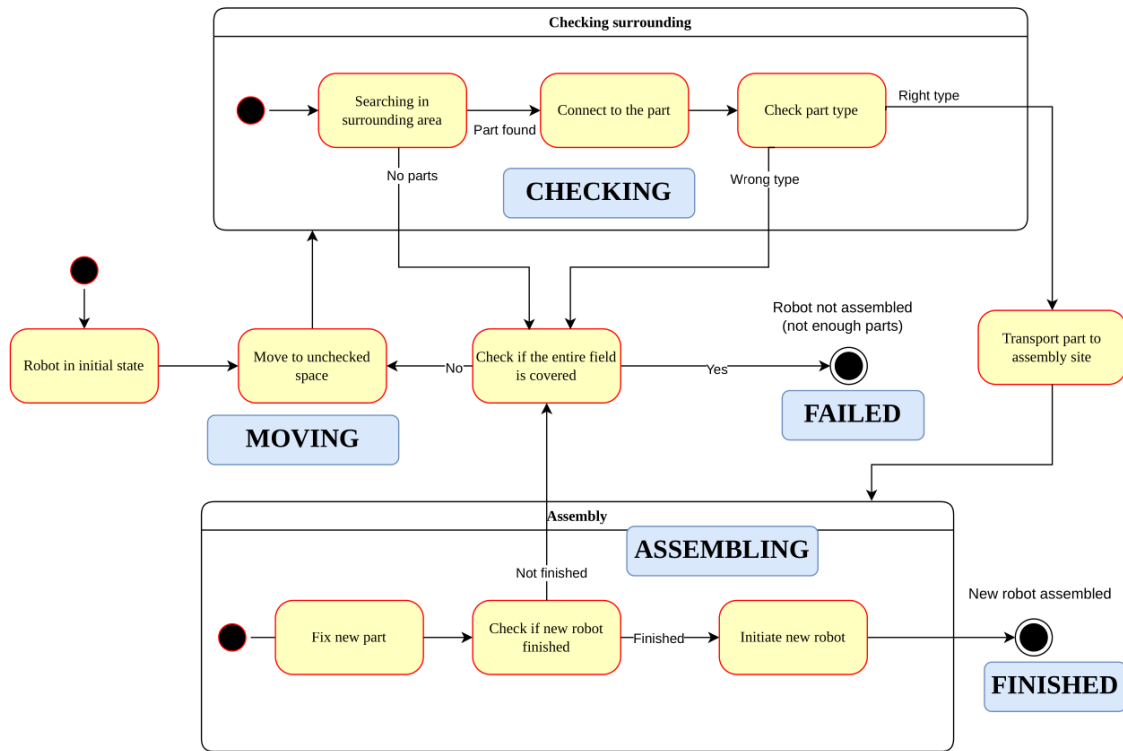
Figure 4.9: State chart of the self-replication system modeled for global reachability
