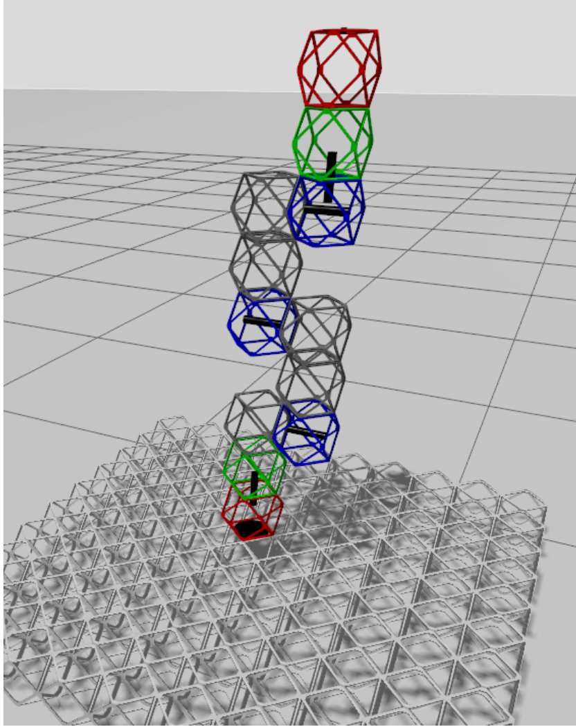
Figure 4.2: Robot structure in Gazebo simulation environment
