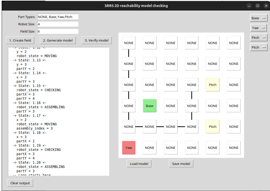
Figure 4.12: Graphical interface for 2D reachability checking with field
