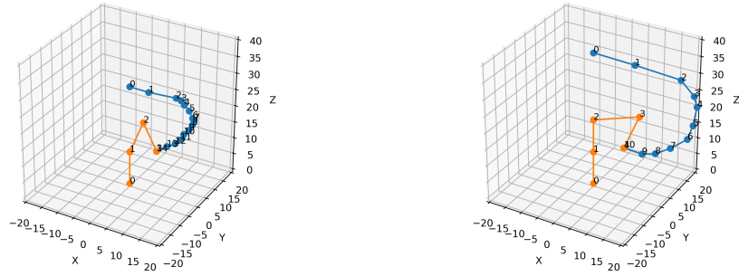
Figure 4.15: Trace for robot length 4 (left) and length 5 (right) for configurations that can reach the target region
