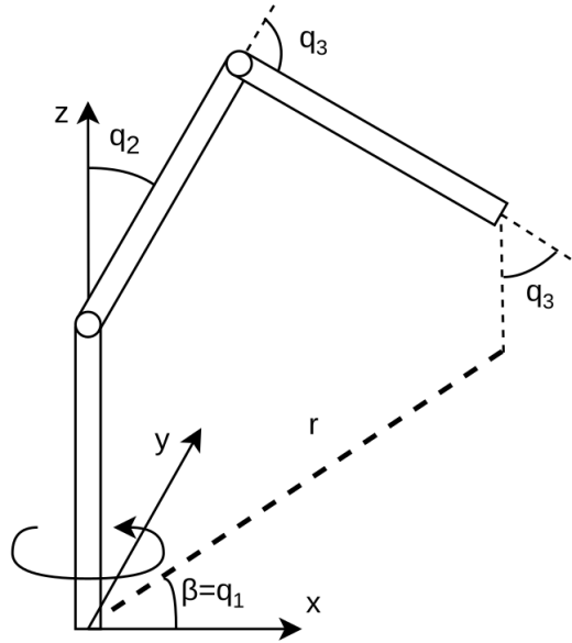
Figure 5.4: Joint angles calculation
