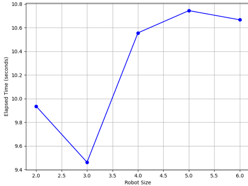
Figure 6.7: Model checking time with robot size
