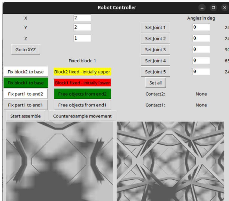
Figure 5.5: Graphical user interface for simulation control
