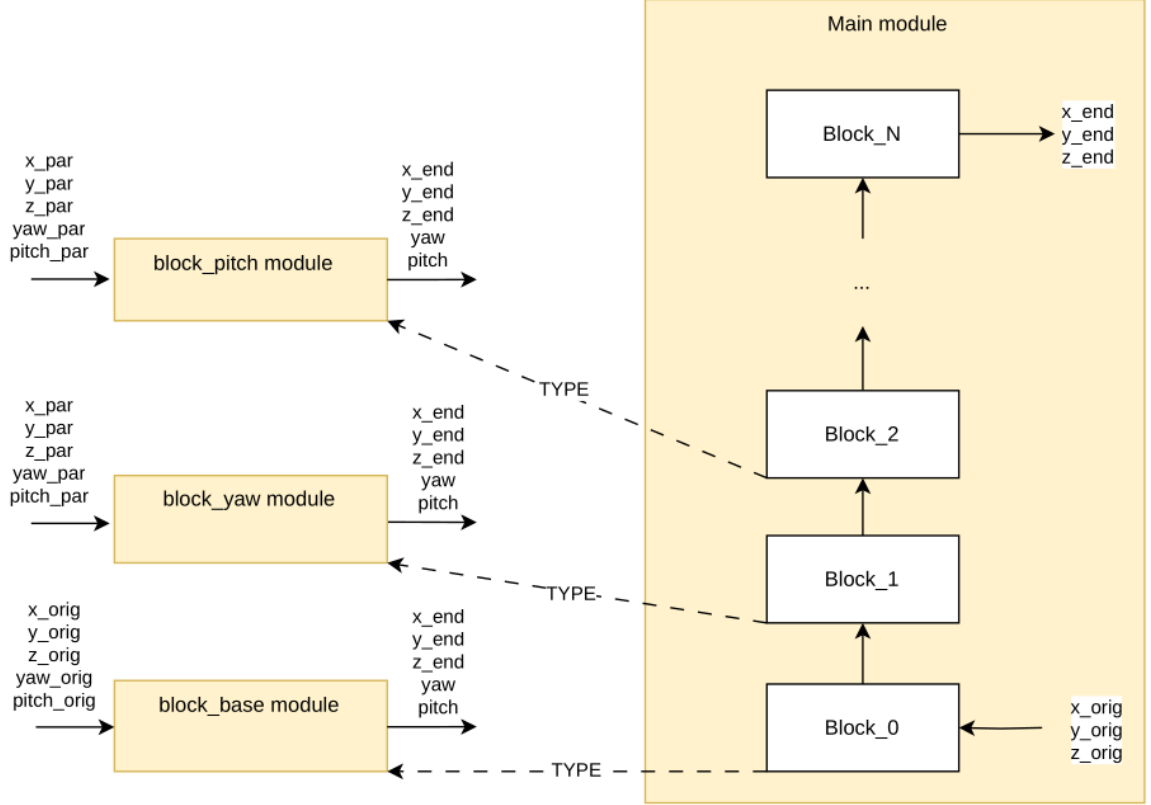
Figure 4.5: Robot configuration NuSMV model
