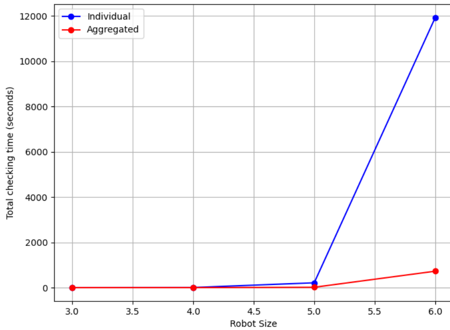
Figure 6.5: Total time of model checking with number of blocks in robot for target region.
