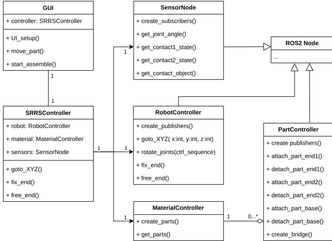
Figure 5.1: Class diagram of the simulation system
