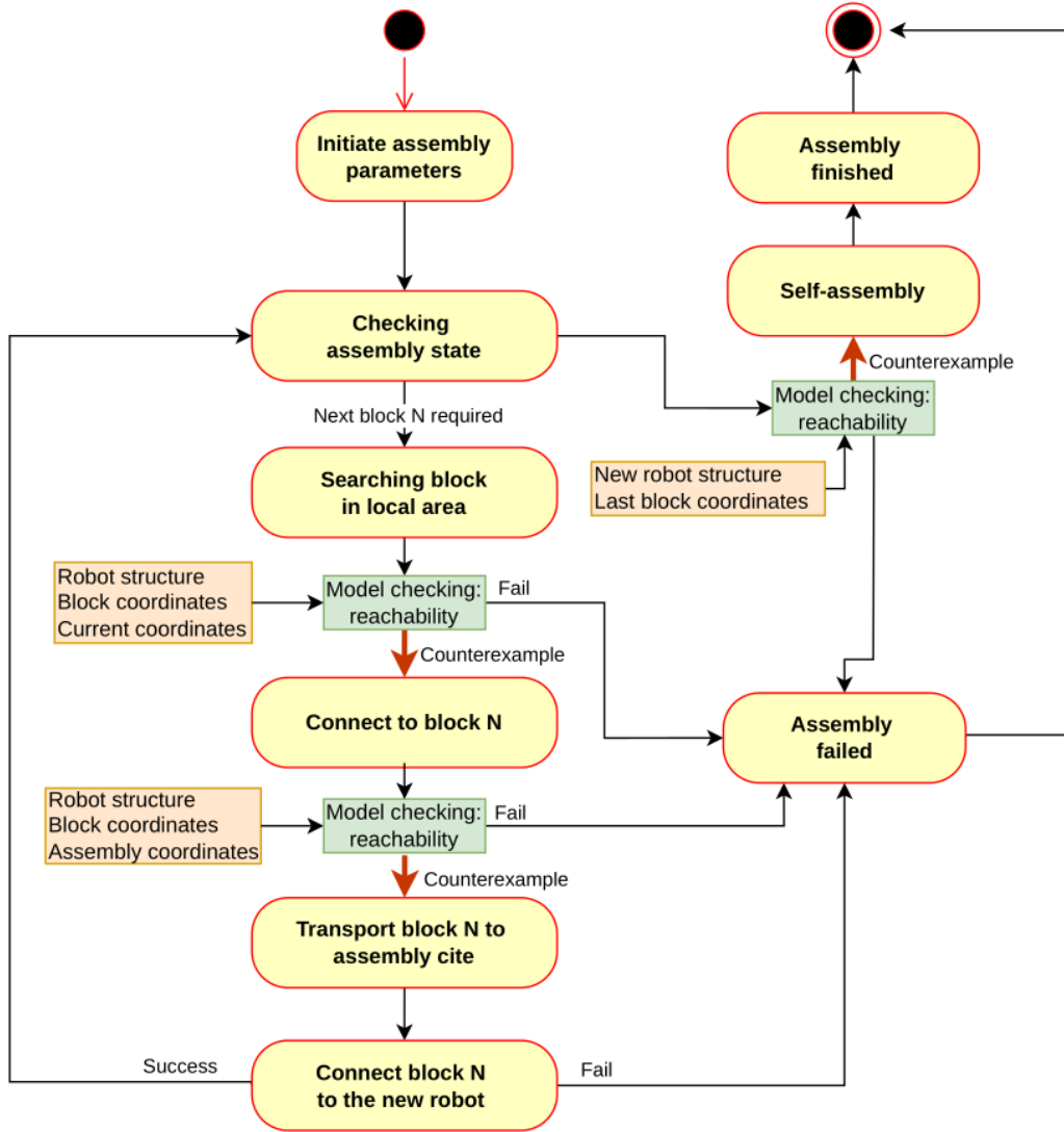
Figure 4.4: Self-replication process with potential model checking stages
