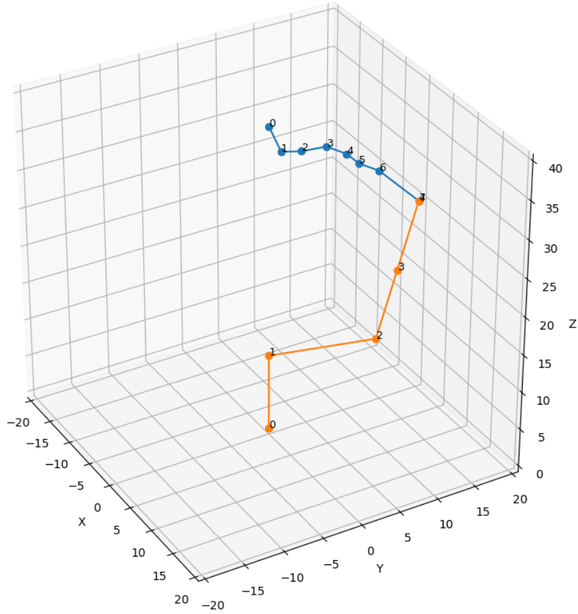
Figure 4.7: Example trace (blue) plot for target point coordinates (10,13,30) and last trace robot position (orange)
