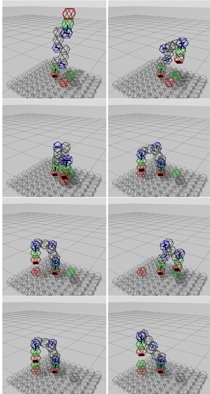
Figure 5.6: Assembly process steps for two initial blocks of a new robot
